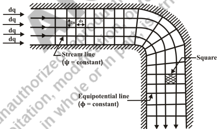
Fig. 4.10 Flow net within a closed conduct
