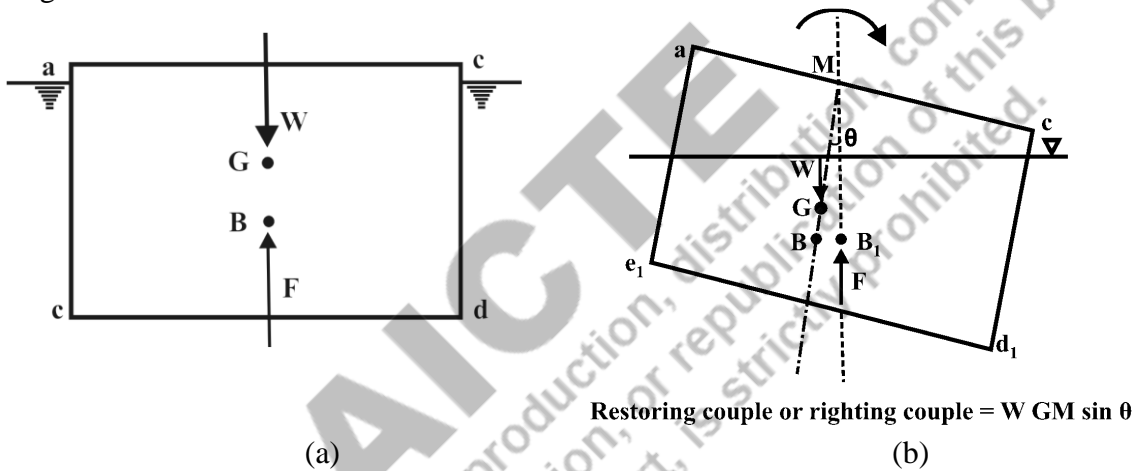
Fig. 3.4 Metacentric height
