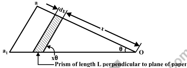
Fig. 3.8 Elementary prism
