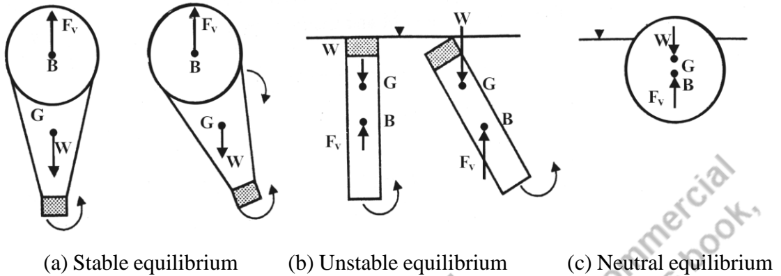
Fig. 3.3 Types of equilibrium
