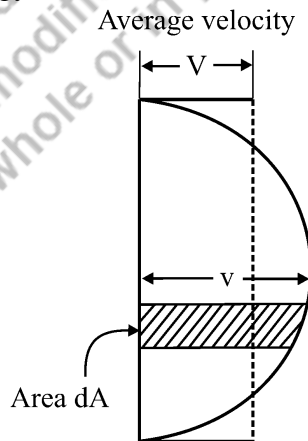
Fig. 5.5 Momentum correction factor ( \beta )
