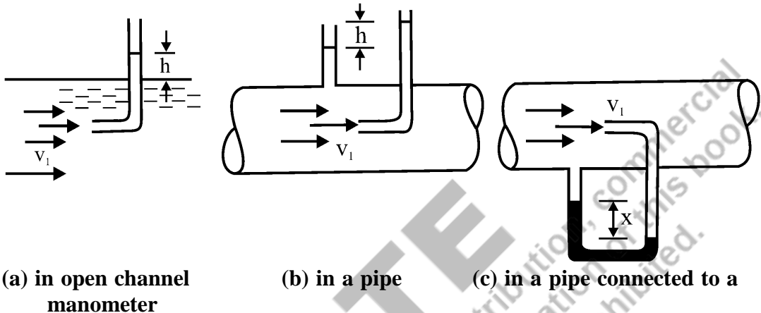
Fig. 5.11 Pitot tube
