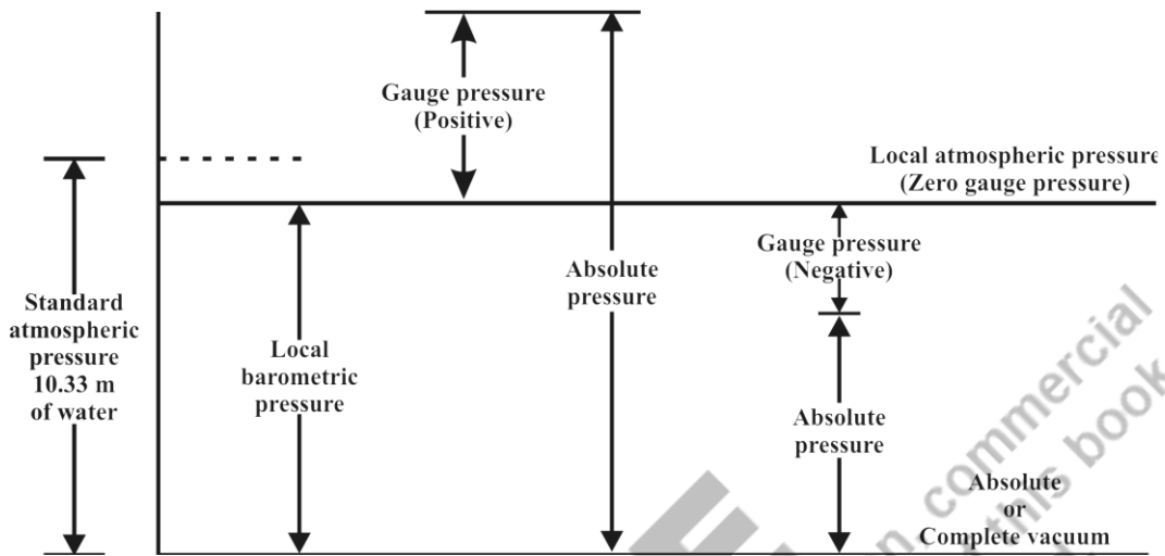
Fig. 2.6 Absolute and gauge pressure
